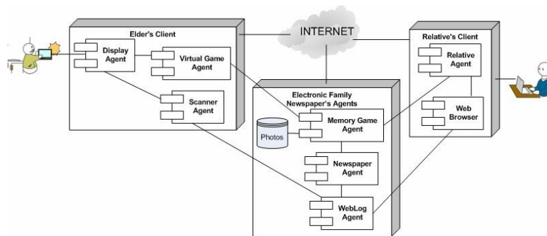
Figure 2. System's components identified as autonomous agents.
